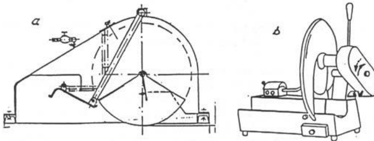
Figure 3.13 a. Deheading machine with a circular saw, operated manually (straight cut), b. Deheading machine with the disc saw and guillotine action (straight cut)
